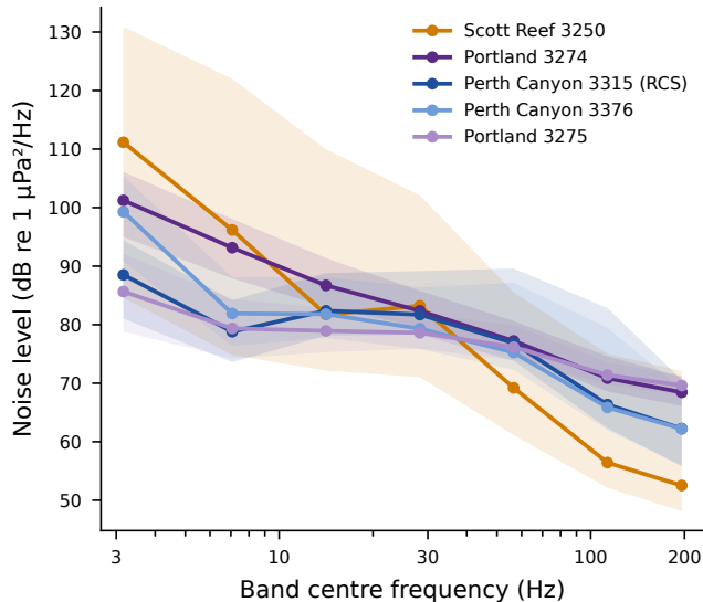
a Background noise: Scott Reef is loud and impulsive below 20 Hz
